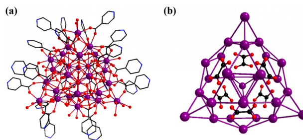
Fig. 1 (a) Plot of the whole molecular structure and (b) the \text{C}_2\text{O}_4^{2-} anion template in the metal skeleton of \text{Gd}_{28} . Purple, Ln; blue, N; red, O; and black, C.
