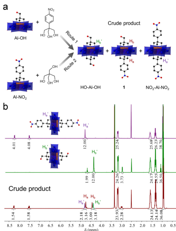
Fig. 1 (a) Schematic representation of the synthetic routes to asymmetric Anderson hybrid 1 . Color code: C, black; N, blue; O, red. The {MoO 6 } octahedron is shown in
