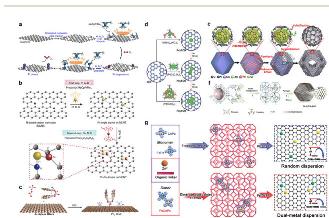
Fig. 3 Schematic diagrams illustrating the synthetic procedure of (a) dimeric Pt 2 /graphene (reproduced with permission from ref. 50 Copyright 2017, Springer Nature), (b) Pt–Ru dimers on nitrogen-doped carbon nanotubes (NCNT) (reproduced with permission from ref. 51 Copyright 2019, Springer Nature), (c) supported Pd 2 DAC (reproduced with permission from ref. 57 Copyright 2021, Wiley-VCH), (d) low-nuclearity Pd catalysts (reproduced with permission from ref. 58 Copyright 2019, Wiley-VCH), (e) hollow carbon-derived nanostructures with porphyrin-like Fe–Co dual sites ((Fe,Co)/N–C) (reproduced with permission from ref. 63 Copyright 2017, American Chemical Society), (f) dual-atom Fe–N 4 /Pt–N 4 sites anchored on the nitrogen-doped carbon matrix (Fe–N 4 /Pt–N 4 @NC) (reproduced with permission from ref. 65 Copyright 2021, Wiley-VCH), and (g) DACs based on the traditional method and the “pre-constrained metal twins” strategy (reproduced with permission from ref. 66 Copyright 2021, Wiley-VCH).
