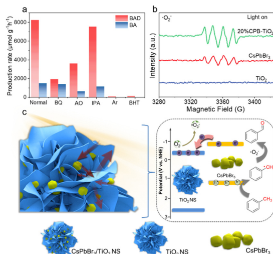
Fig. 8 (a) Photocatalytic toluene oxidation in the absence or presence of various radical scavengers. (b) EPR spectra of \text{DMPO} \cdot \text{O}_2^- . (c) Schematic illustration of the proposed mechanism of photocatalytic oxidation of toluene over the \text{CPB/TiO}_2 composite.
