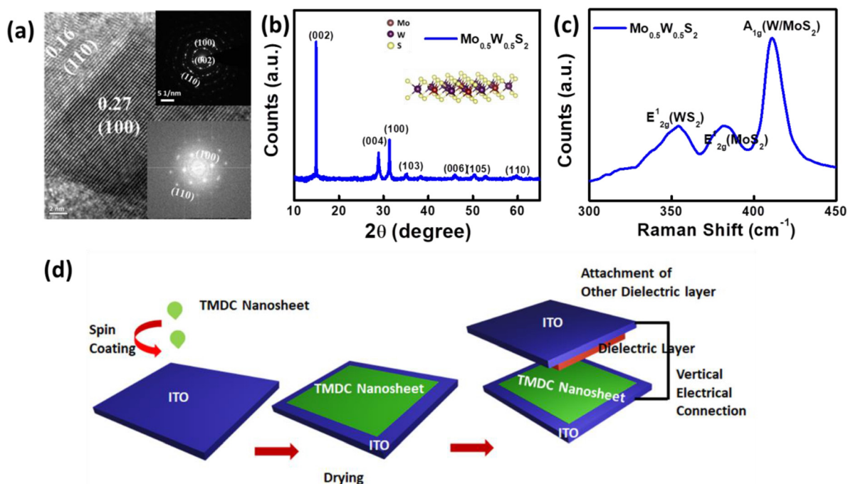
Fig. 1 (a) High-resolution TEM image of the Mo 0.5 W 0.5 S 2 nanosheet with interlayer spacings, with the inset showing the corresponding FFT and SAED patterns of the nanosheet. (b) XRD pattern of the Mo 0.5 W 0.5 S 2 alloy nanosheet, with the schematic of the structure shown in the inset. (c) Typical Raman spectra of the alloy nanosheet at an excitation wavelength of ~532 nm, with the indexed vibrational modes indexed. (d) Schematic steps for the fabrication of vertical-mode TENG devices.
