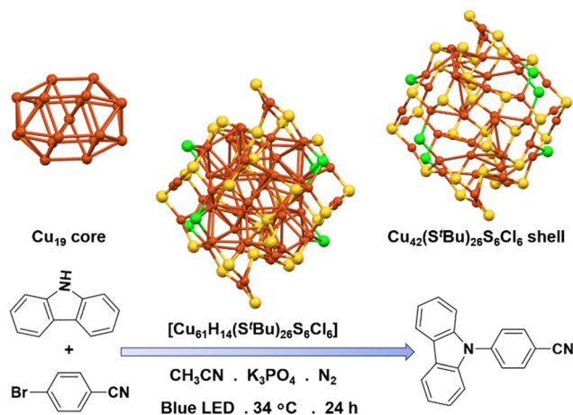
Fig. 7 Structural architecture of [\text{Cu}_{61}\text{H}_{14}(\text{SiBu})_{26}\text{S}_6\text{Cl}_6] NC and its effectiveness towards photocatalytic C–N coupling reaction. Cu displayed in brown color; S displayed in yellow color and Cl displayed in green color. Other ligands were removed for clarity. Hydrides were not detected by SCXRD. Figure created based on the cif file deposition of ref. 73.
