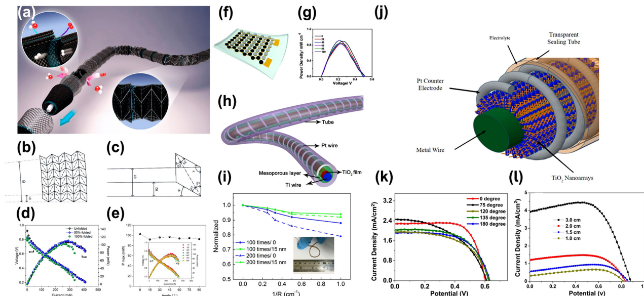
Fig. 13 (a) Schematic of the flexible origami tubular PEMFC. Illustration of (b) angle \theta corresponding to the overall angle of the origami component and (c) the detailed geometric parameters of a single origami cell. (d) Polarization curves of the kirigami tubular PEMFC under unfolded, 50%-folded and 100%-folded states. (e) Variation of maximum power with bending angle, inset: polarization curve of the kirigami tubular PEMFC at various bending angles. (f) Schematic of the stretchable island-bridge structure, E-BFC. (g) Polarization curve of the island-bridge structure E-BFC under increasing stretching deformation with strain of 50%. (h) Schematic of the FDSSC with \text{TiO}_2 film coated on anode. (i) Comparison of power conversion efficiency (PCE) of the FDSSC with ALD \text{TiO}_2 films of different thickness, tested at different bending curvature and bending times. (j) Schematic of the FDSSC with 1D \text{TiO}_2 nanowire arrays on the anode. Comparison of photovoltaic performances of the FDSSCs tested with (k) varying bending angles and (l) with increasing length. Reproduction with permission from ref. 107, Copyright 2021, American Chemical Society and Reproduction with permission from ref. 108, Copyright 2017, Royal Society of Chemistry and Reproduction with permission from ref. 109, Copyright 2016, Springer Nature Limited and Reproduction with permission from ref. 110, Copyright 2021, Springer Nature Limited.
