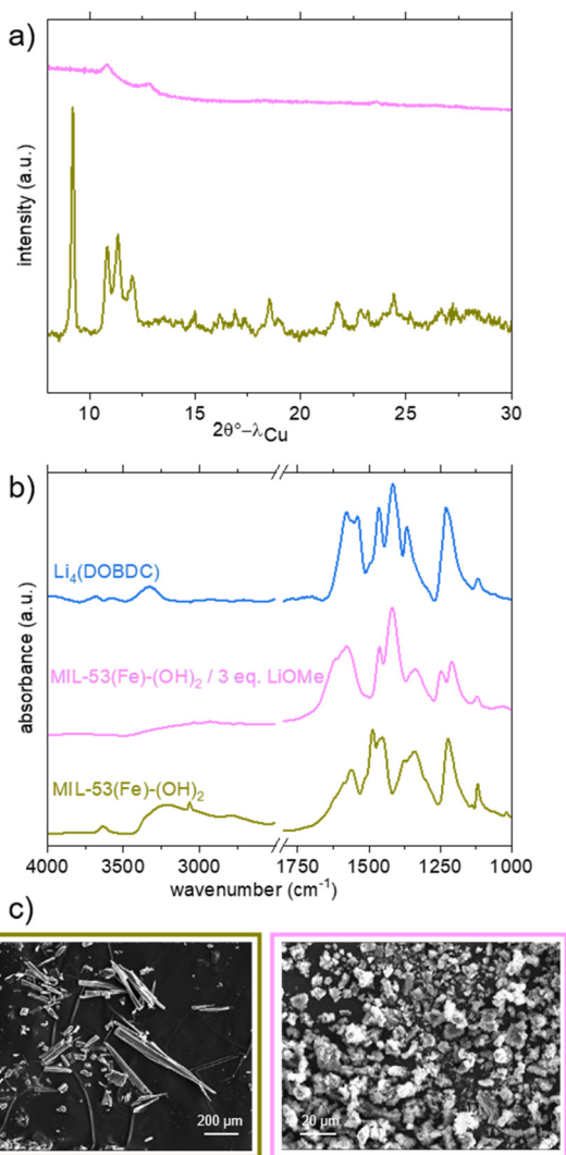
Fig. 5 Characterisation of \text{MIL-53(Fe)-(OH)}_2 and its lithiated product from LiOMe in MeOH/THF. a) PXRD patterns ( \lambda = 1.5406\text{ Å} ); b) IR spectra; c) SEM pictures. Data related to dry \text{MIL-53(Fe)-(OH)}_2 , \text{Li}_4(\text{DOBDC}) and the lithiation product are shown in khaki, blue and pink, respectively.
