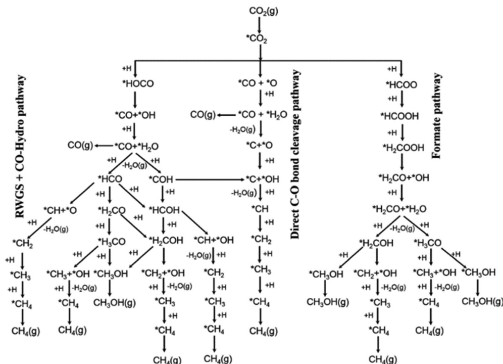
Fig. 3 Possible reaction pathways of CO 2 hydrogenation to CO, CH 3 OH, and CH 4 . *(X) indicates adsorbed species. Reprinted with permission from ref. 57. Copyright 2017 American Chemical Society ( https://pubs.acs.org/doi/10.1021/jacs.7b05362 ).
