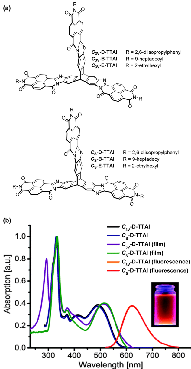
Fig. 9 (a) Molecular structures of triptycene-trisaroylenimiazoles; (b) \text{CH}_2\text{Cl}_2 solution absorbance and emission spectra and thin film absorbance spectra of C 3V -D-TTAI and C 3V -D-TTAI . Reproduced from ref. 58 with permission from the Royal Society of Chemistry.
