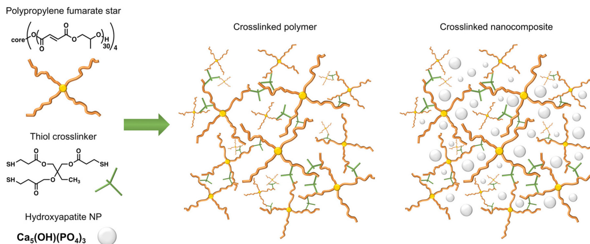
Fig. 1 Poly(propylene fumarate) 4-arm star polymers were crosslinked photochemically using a Carbon M2 printer and a crosslinker with three pendant thiol groups. Hydroxyapatite nanopowder was added to the resin and printed to yield nanocomposites. Tensile bars, DMA bars, and gyroid scaffolds were 3D printed and subjected to different post-curing conditions.
