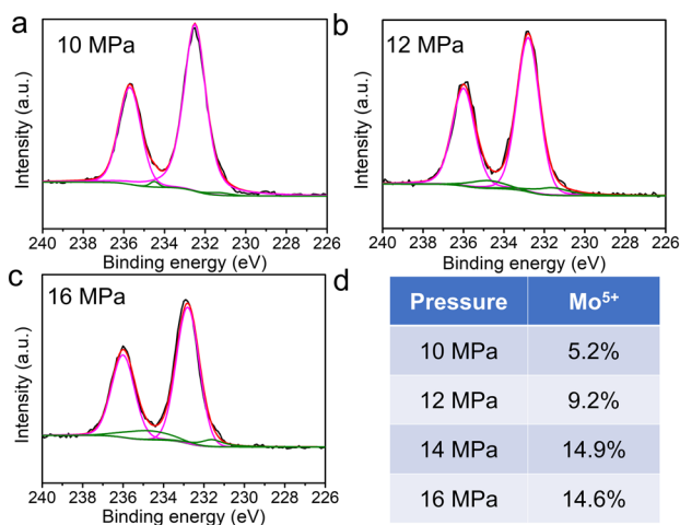
Fig. 5 (a-c) XPS spectrum details of the Mo 3d binding energy regions and (d) the varied percent of \text{Mo}^{5+} for the \text{MoO}_{3-x} sample obtained at 10 MPa, 12 MPa, 14 MPa, 16 MPa.
