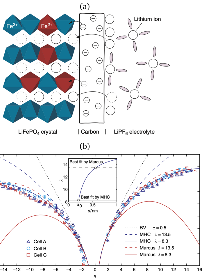
Fig. 3 Kinetics of lithium intercalation in lithium iron phosphate (LFP). (a) Reaction mechanism defined here as “electron-coupled ion transfer (ECIT)”, in which ion insertion is limited by electron transfer from the carbon coating to reduce a neighboring iron redox site and form a neutral polaron. (b) Evidence for Marcus kinetics in LFP from Tafel plots of the rate constant for reaction-limited nanoparticle phase transformations versus dimensionless overpotential (scaled to k_B T/e = 26 mV), fitted to the Marcus–Hush–Chidsey (MHC) model. [Reproduced from Bai and Bazant (2014). 63 ]
