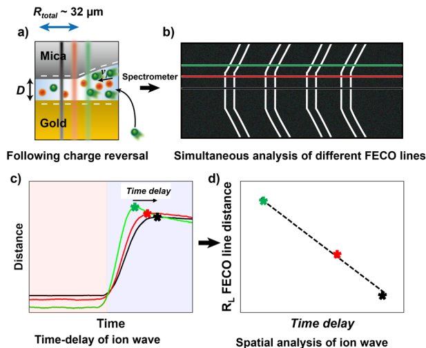
Fig. 3 More detailed explanation of observed phenomenon. (a) Schematics of the spatial resolution of the ion transport based on charge reversal of the gold surface. (b) FECo lines with highlighted lines used to observe the ion wave. (c) Time-dependent distance measurement during ion exchange. The centre line (black) has a time delay in relation to the outer lines (green, red) in distance change due to the ion transport. This is observable due to the high-speed resolution of the spectrograph. (d) Relation of time delay of ion wave and spatial distance of FECo line to the centre. This curve allows analysing ion speed in a confined gap.
