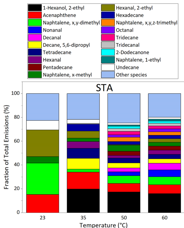
Fig. 6 Evolution of VOC emission composition in % for the species accounting for more than 75% of VOC emissions ( EF > 3.49 \mu g m^{-2} h^{-1} for STA asphalt mixtures) as a function of temperature, as measured by GC-MS/FID under dry ( RH = 0.1\% ) and dark conditions, for the STA3 fresh asphalt sample.
