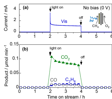
Fig. 9 PEC oxidation of CH 4 by the PEM-PEC reactor using the WO 3 photoanode and Pt/carbon catalyst: (a) the overall current at zero bias, and (b) the rate of products formation on the photoanode side under 453 nm light irradiation (6.8 mW cm -2 ).
