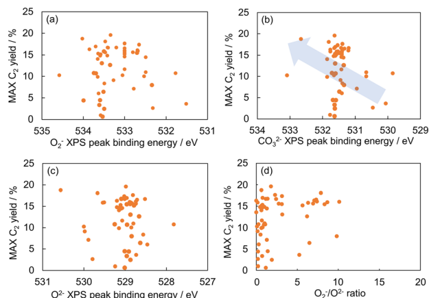
Fig. 1 Plots of maximum C 2 yield against the three deconvoluted O1s XPS peaks assignable to (a) O 2 •− , (b) CO 3 2− , and (c) O 2 2− species. (d) Plot of maximum C 2 yield against O 2 •− /O 2 2− ratio. Maximum C 2 yield: the highest C 2 yield value obtained with each catalyst in the experiment protocol.
