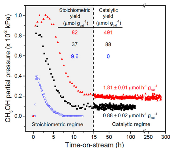
Fig. 11 Catalytic performance of Cu-ZSM-5 in the partial oxidation of methane. Pretreatment conditions: \text{O}_2 flow at 823 K for 5 h. Reaction conditions (chemical looping) for Cu-Na-ZSM-5 (blue open squares, \text{Cu}/\text{Al} = 0.37 , \text{Na}/\text{Al} = 0.26 ): reaction with methane, \text{WHSV} = 2400 \text{ mL h}^{-1} \text{g}_{\text{cat}}^{-1} , 483 K, 0.5 h; extraction of methanol, \text{WHSV} = 2400 \text{ mL h}^{-1} \text{g}_{\text{cat}}^{-1} , 483 K, P_{\text{He}} = 98.1 \text{ kPa} , P_{\text{H}_2\text{O}} = 3.2 \text{ kPa} , P_{\text{O}_2} = 0.0025 \text{ kPa} . Reaction conditions (continuous-flow) for Cu-Na-ZSM-5 (black filled squares) and Cu-H-ZSM-5 (red filled triangles, \text{Cu}/\text{Al} = 0.31 ): \text{WHSV} = 2400 \text{ mL h}^{-1} \text{g}_{\text{cat}}^{-1} , 483 K, P_{\text{CH}_4} = 98.1 \text{ kPa} , P_{\text{H}_2\text{O}} = 3.2 \text{ kPa} , P_{\text{O}_2} = 0.0025 \text{ kPa} . Reprinted from ref. 50 with permission from American Chemical Society, copyright 2016.
