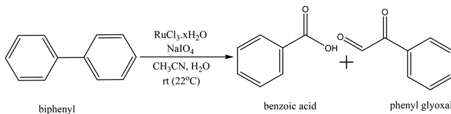
Scheme 1 Ruthenium ion catalysed oxidation of biphenyl to benzoic acid.
