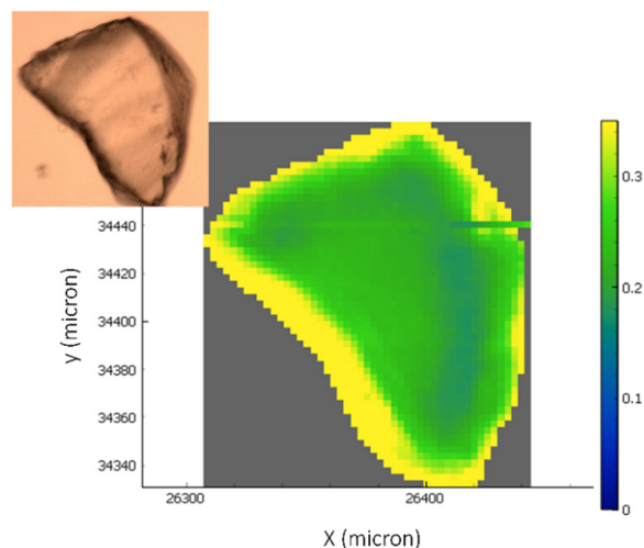
Fig. 4 The optical image of the carriers with the overlap of the chemical infrared image generated by the ratio of the integration in the specific region of amide I and amide II bands (~1710–1480 cm -1 ) and the band identifying the glass carrier (~1500–1300 cm -1 ). The colour scale bar ranges from higher biocatalyst concentrations (yellow areas) to not-detectable concentrations (blue areas).
