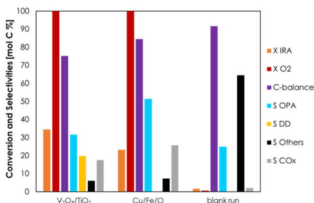
Fig. 1 ODH of IRA over V_2O_5/TiO_2 , Cu/Fe/O and without any catalyst. Reaction conditions: volume of catalyst = 1 \text{ cm}^3 , temperature = 300 °C, IRA/ O_2/N_2 = 5/5/90 mol%, contact time ( \tau ) = 1 second. Symbols: Isorosalva Alcohol conversion ( X_{IRA} , orange), oxygen conversion ( X_{O_2} , dark red), carbon balance (C-balance, purple), opalene selectivity ( S_{OPA} , light blue), decadiene selectivity ( S_{DD} , yellow), other by-products' selectivity ( S_{Others} , black) and CO_x selectivity ( S_{CO_x} , grey). Mean values calculated at the steady-state during the last 3 h of time on stream.
