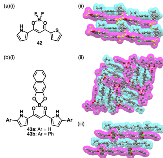
Fig. 29 (a) (i) Pyrrolylthienyldiketone BF_2 complex 42 and (ii) single-crystal X-ray structure of {}^3TATA^+-42\cdot Cl^- and (b) (i) naphthalenediolate boron complexes 43a,b and (ii) single-crystal X-ray structures of {}^3TATA^+-43a\cdot Cl^- and (iii) {}^3TATA^+-43b\cdot Cl^- . The crystal structures are redrawn from cif files: 1840326, 2227398 and 2227399.
