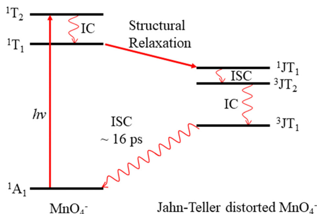
Fig. 1 Excitation of \text{MnO}_4^- in the visible to ^1T_2 , followed by rapid relaxation via the ^3T_1 state of a Jahn–Teller distorted \text{MnO}_4^- back to ^1A_1 , via structural relaxation, internal conversion (IC) and intersystem crossing (ISC). The transition from ^1A_1 to ^1T_1 is symmetry forbidden.
