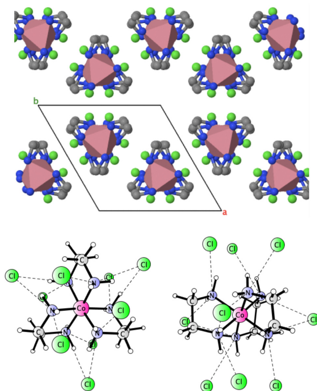
Fig. 5 Crystal structure of [\text{Co}(\text{en})_3]\text{Cl}_3 viewed along the crystallographic axis c (H atoms not shown for clarity) and two views on the \{[\text{Co}(\text{en})_3]\text{Cl}_9\}^{6-} cluster excised from the crystal structure. The N(H)···Cl close contacts are indicated with dashed lines.
