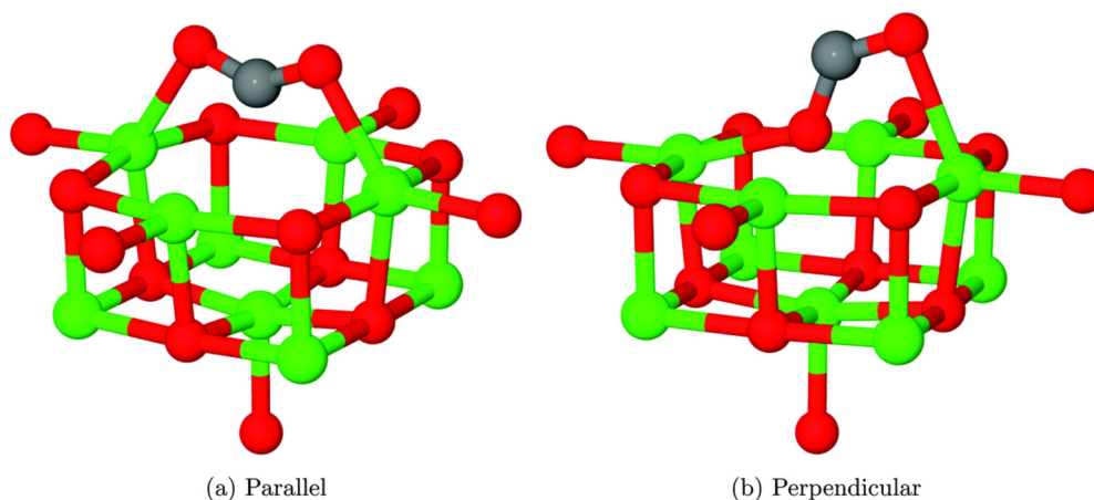
Fig. 13 Parallel and perpendicular adsorption modes of CO 2 adsorption on an MgO surface with an F^{\cdot} defect containing two localised electrons. Figure reprinted from ref. 194 under a Creative Commons license (CC BY 3.0).
