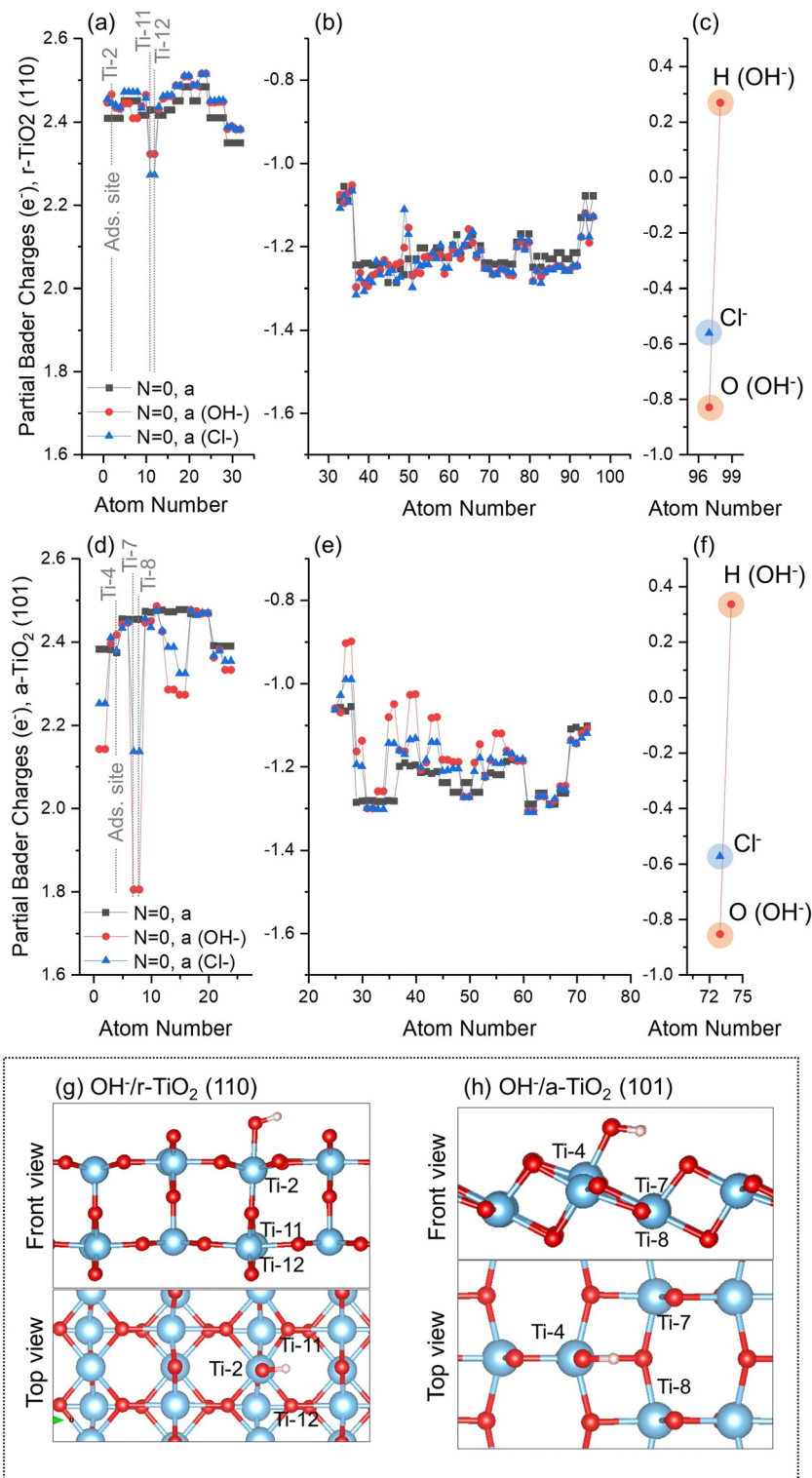
Fig. 4 Partial Bader charges for ground state (singlet, N = 0 ) electronic structure of clean, hydroxyl-, and chloride-containing (a–c) r -TiO _2 (110) and (d–f) a -TiO _2 (101) surfaces. Charges over Ti ions (a and d), O ions (b and e), and adsorbates (c and f) are individually presented. Inserts show representative example of adsorbate-containing surface (g: OH ^- /r-TiO _2 (110); h: OH ^- /a-TiO _2 (101)). Atom numbers refer to labels defined in the methodology section.
