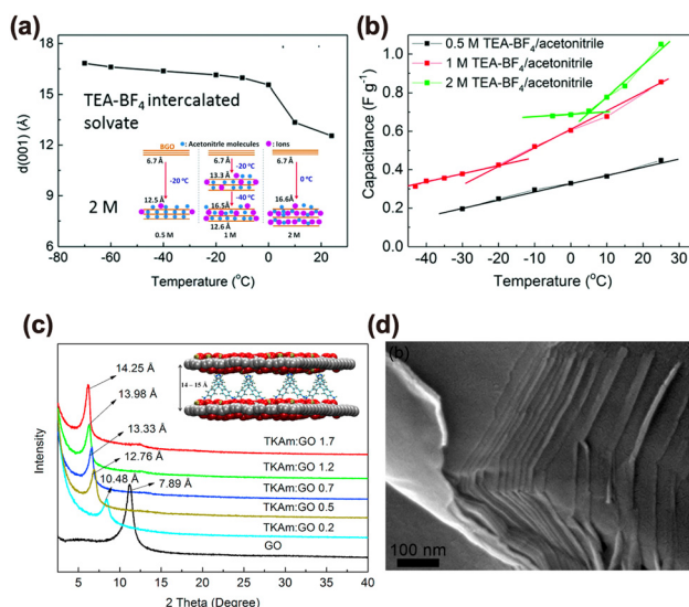
Fig. 3 Examples of GRMs used to boost the ionic conductivity of electrode materials. (a) Temperature dependence of the (001) d -spacing for BGO in 2 M TEA- \text{BF}_4 electrolyte. The inset shows a scheme of the interlayer spacing adjustment via temperature- and concentration-dependent intercalation of solvated TEA- \text{BF}_4 ions into BGO. (b) Comparison of the specific capacitances of BGO electrodes in 0.5, 1, and 2 M TEA- \text{BF}_4 /acetonitrile under various temperatures. Reproduced with permission. 23 Copyright 2018, Royal Society of Chemistry. (c) XRD patterns of the samples with various loading of TKAm:GO. The inset shows a schematic illustration of the pillared GO/TKAm structure. (d) SEM image of the H-GO/TKAm sample grain edges. Reproduced with permission. 24 Copyright 2017, Elsevier.
