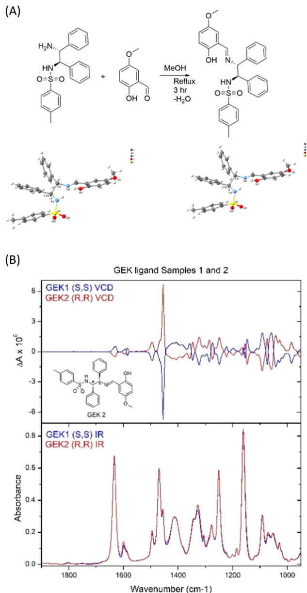
Fig. 3 (A) Synthesis of 1(S),2(S)-N,N chiral ligand for catalysis and projection of the crystal structure of the chiral (S)-, (S)- (left) and (R)-, (R)- (right) organic ligands. (B) VCD spectra of (R)-, (R)- and (S)-, (S)- ligands.
