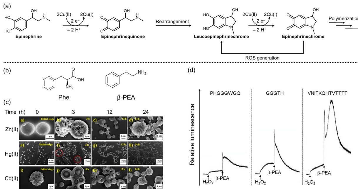
Fig. 4 Structural changes of epinephrine as well as fibrilization and ROS generation of Phe and β-PEA in the presence of divalent metal ions. (a) Oxidation and polymerization of epinephrine in the presence of \text{Cu(II)} . (b) Chemical structures of Phe and β-PEA. (c) Aggregation of Phe into fibrillar species in the presence of divalent metal ions, including \text{Zn(II)} , \text{Cd(II)} , and \text{Hg(II)} . Reproduced with permission from ref. 141. Copyright © 2022 American Chemical Society. (d) Increased levels of \text{O}_2^{\bullet-} by incubation of β-PEA, \text{Cu(II)} , and fragments of the prion protein. Reproduced with permission from ref. 142. Copyright © 2006 Ivyspring International Publisher.
