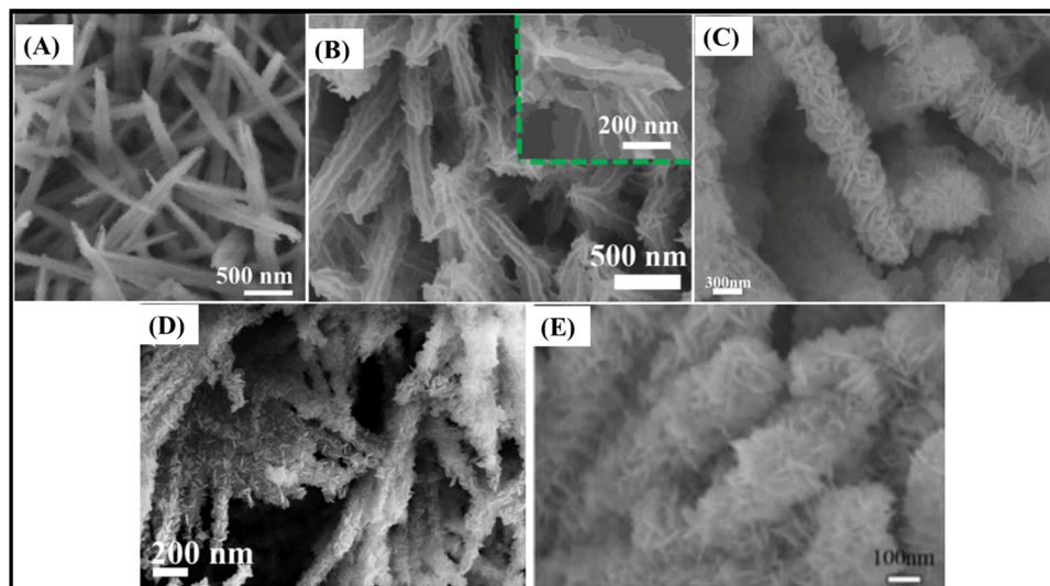
Fig. 8 SEM images of (A) \text{ZnCo}_2\text{O}_4@\text{NiMoO}_4 heterostructured nanowires/NF, 119 (B) \text{ZnCo}_2\text{O}_4@\text{NiMoO}_4 heterostructured nanowires/NF, 120 (C) \text{r-ZnCo}_2\text{O}_4@\text{NiMoO}_4\cdot\text{H}_2\text{O} heterostructured nanowires/NF, 121 (D) \text{ZnCo}_2\text{O}_4@\text{ZnWO}_4 heterostructured nanowires/NF 123 and (E) \text{ZnCo}_2\text{O}_4@\text{NiWO}_4 heterostructures/NF. 124 Panel A: Reproduced with permission. 119 Copyright © 2020 Elsevier Ltd. All rights reserved. Panel B: Reproduced with permission. 120 Copyright © 2020 Elsevier Ltd. All rights reserved. Panel C: Reproduced with permission. 121 © 2018 Elsevier B.V. All rights reserved. Panel D: Reproduced with permission. 123 Copyright © 2018 Published by Elsevier Inc. Panel E: Reproduced with permission. 124 Copyright © 2020, Springer-Verlag GmbH Germany, part of Springer Nature.
