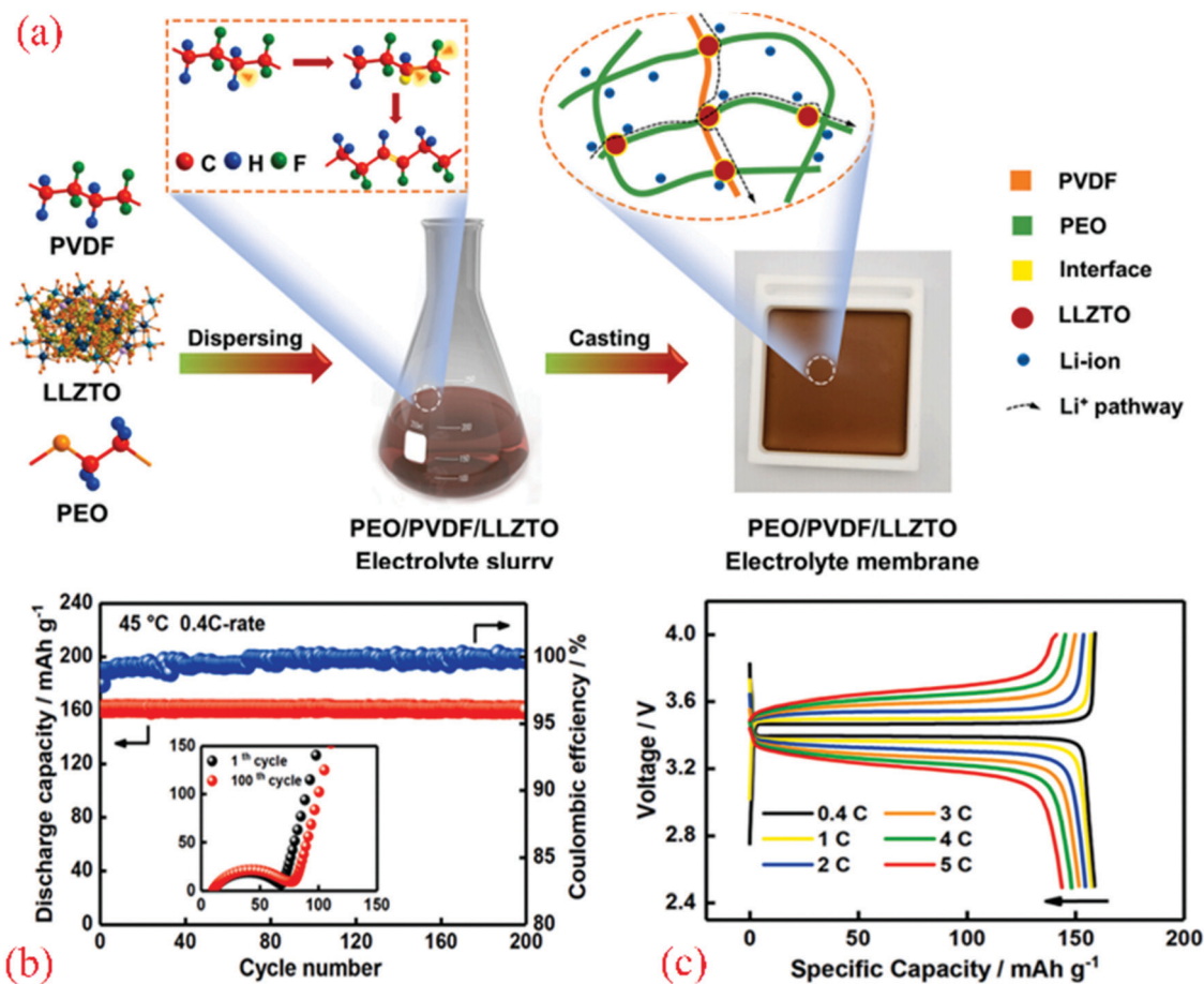
Fig. 21 (a) Fabrication process of the PLFF (PEO/PVDF/LLZTO/LiTFSI) solid composite electrolyte. (b) Cycling performances at 0.4C and 45 °C and the impedance of LiFePO 4 /Li cell cycling with PLFF. (c) Different rates of galvanostatic charge–discharge profiles of LiFePO 4 /PLFF/Li cells under 45 °C. 358 Reproduced with permission from Elsevier. 358
