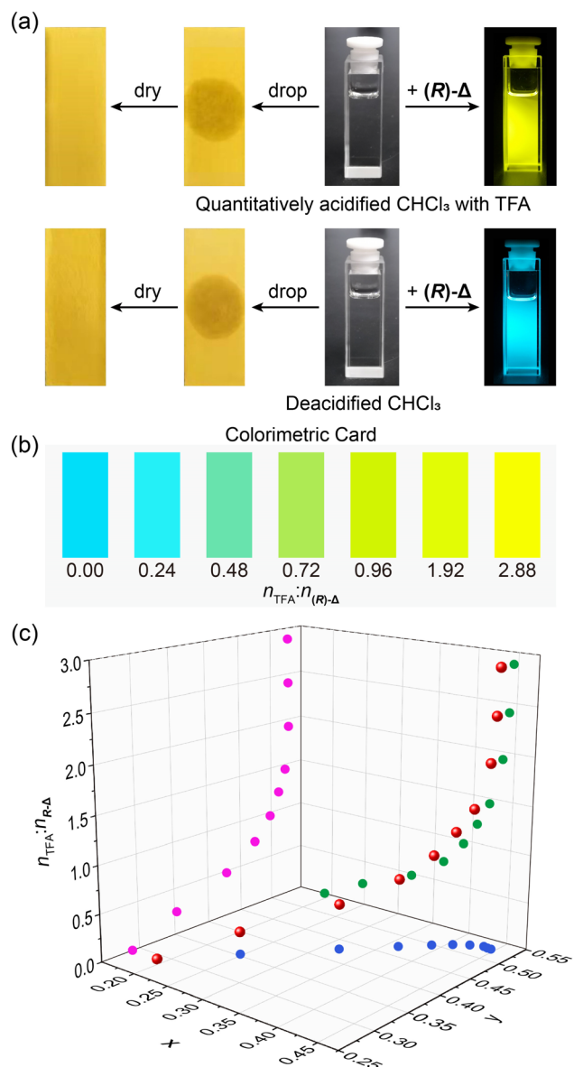
Fig. 4 Detecting traces of acids employing (R)-Δ. (a) Fluorescence changes of solutions (right) of (R)-Δ in \text{CHCl}_3 with and without TFA upon shining 365 nm-UV light in comparison with detecting trace acid in the same solvents using pH papers (left). (b) A colorimetric card showing the ability of (R)-Δ to detect visually amounts of acid in solutions with different n_{\text{TFA}}:n_{(\text{R})-\Delta} ratios. (c) The fitting function based on the PL emission of (R)-Δ upon changing the n_{\text{TFA}}:n_{(\text{R})-\Delta} ratio from 0.00 to 2.88. The concentration of (R)-Δ is 1 \times 10^{-5} M.
