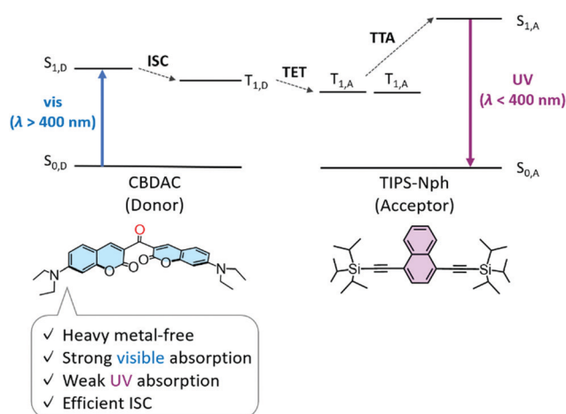
Fig. 1 Energy level diagram of vis-to-UV TTA-UC using a heavy metal-free donor CBDAC and an acceptor TIPS-Nph.
