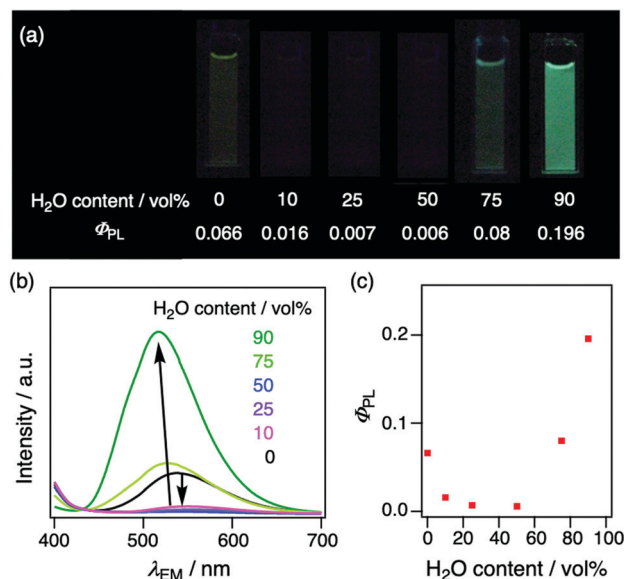
Fig. 5 (a) Photographs taken under blacklight ( \lambda_{\text{EX}} = 365 nm), (b) PL spectra, and (c) plots of absolute \Phi_{\text{PL}} against H 2 O content (vol%) in THF solution of 2Cz2SB ( 2 \times 10^{-5} M).
