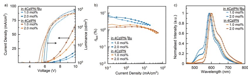
Fig. 4 (a) Comparison of current density–voltage–luminance ( J – V – L ) characteristics, (b) comparison of EQEs versus current densities, and (c) comparison of EL at EQE max for OLED with binary blend EML.
