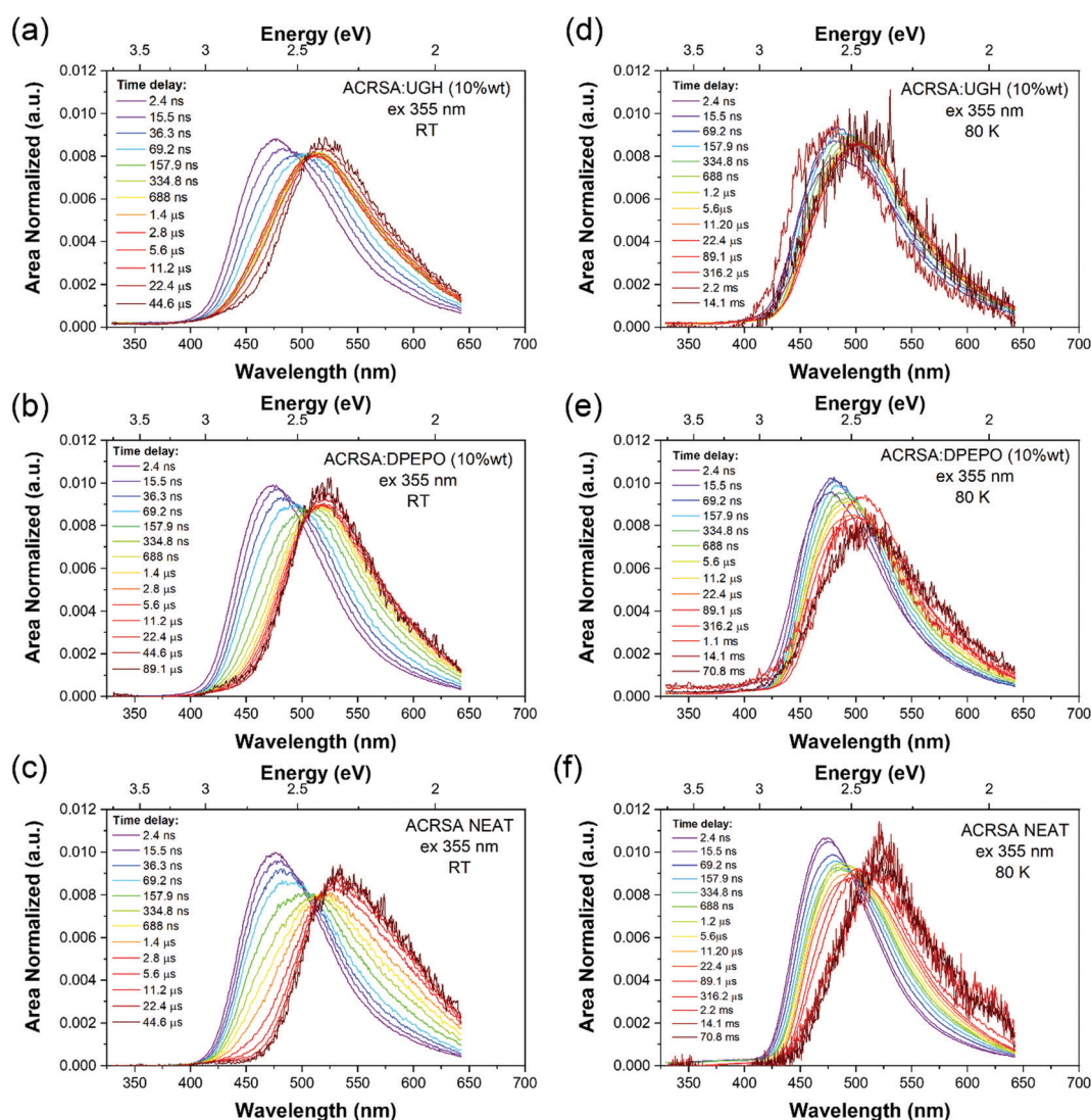
Fig. 4 Time evolution of the emission spectra (area normalised). Laser excitation at 355 nm excitation wavelength, for ACRSA in UGH, DPEO (10% loading) and neat film measured at; (a–c) 300 K, (d–f) at 80 K. Normalised data shown in Fig. S25 (ESI†).
