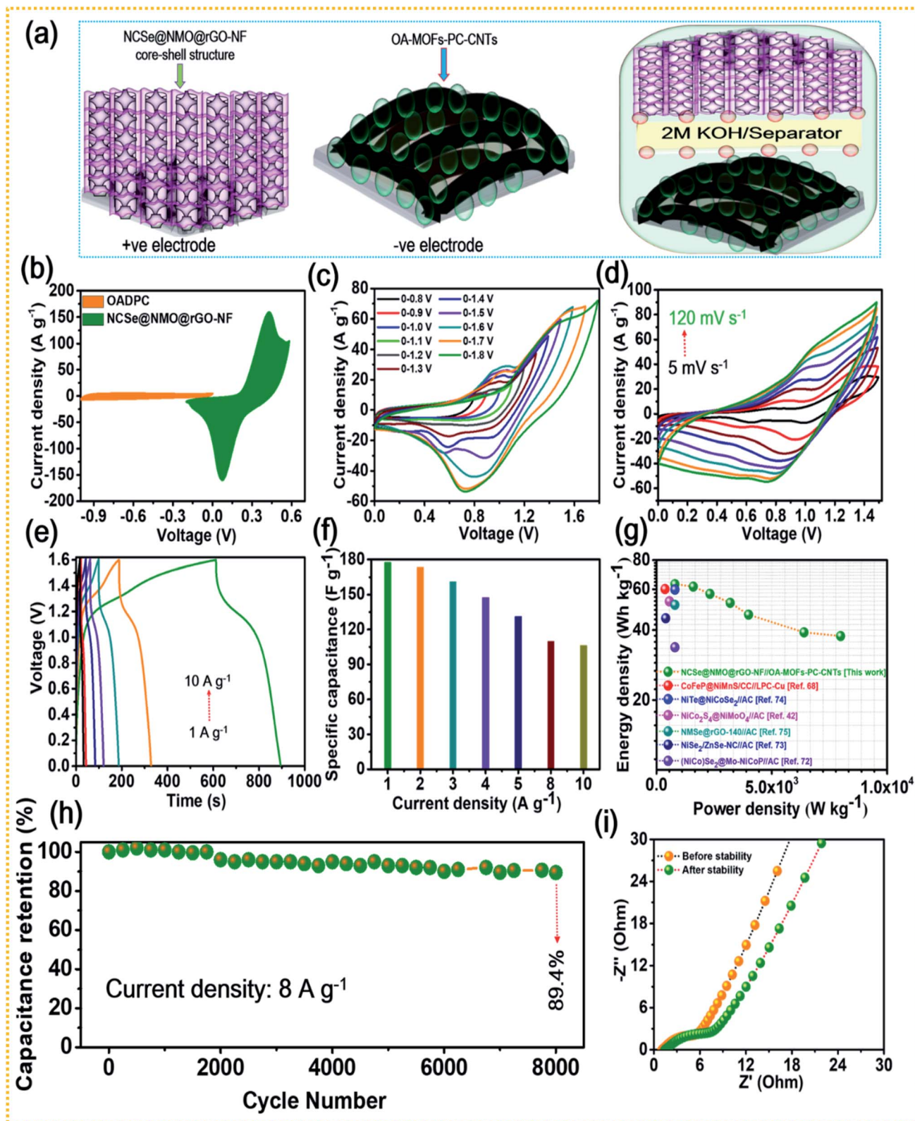
Fig. 7 (a) Schematic representation of the HSC device, (b) CV curves of the NCSe@NMO@rGO-NF and OA-MOFs-PC-CNTs electrodes, (c) CV curves of the HSC device at different potentials, (d) CV curves recorded at different scan rates, (e) GCD curves recorded at various current densities, (f) rate capability data of the HSC device, (g) Ragone plot showing the energy and power densities of the HSC device, (h) cycling stability of the HSC, and (i) EIS curves of the HSC device tested before and after the cycling stability tests.
