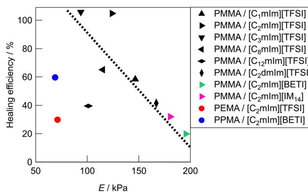
Fig. 5 Relationship between the Young's modulus ( E ) and the healing efficiency of UHMW gels. The dotted line is a guide to the eye. The healing efficiency was defined as the ratios of mechanical toughness (the area under the stress–strain curve) between pristine and healed gels.
