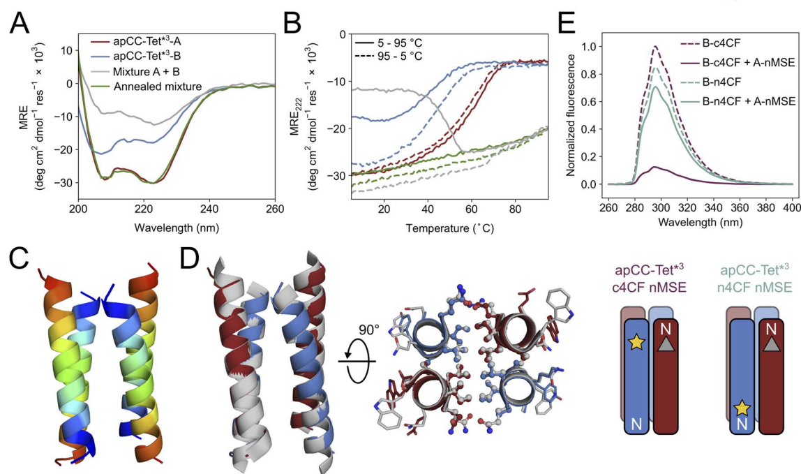
Fig. 4 Biophysical and structural characterization of the heterotetrameric complex apCC-Tet * - A_2B_2 . (A) CD spectra at 5 °C and (B) thermal response curves (ramping up, solid lines; and ramping down, dashed line) for apCC-Tet * -A (red), apCC-Tet * -B (blue), the pre-annealed mixture apCC-Tet * - A_2B_2 (grey), and the annealed mixture apCC-Tet * - A_2B_2 (green). Conditions: 50 \mu M peptide, PBS, pH 7.4. (C) X-ray crystal structure of the heteromeric assembly apCC-Tet * - A_2B_2 (PDB ID: 8a3j) with the chains coloured from the N (blue) to the C termini (red). (D) Alignment of the crystal structures of apCC-Tet * - A_2B_2 (apCC-Tet * -A, red; apCC-Tet * -B, blue) and the related homotetramer apCC-Tet * (grey). (E) Fluorescence-quenching assay for labelled apCC-Tet * - A_2B_2 peptides. 4CF is the 4-cyano-L-phenylalanine fluorophore (yellow star) and MSE is the L-selenomethionine fluorescence quencher (grey triangle). 'n' and 'c' indicate mutations near the N and C termini, respectively. In this panel only, peptide names are shortened for clarity. Conditions: 50 \mu M concentration of each peptide in phosphate buffer (8.2 mM sodium phosphate dibasic, 1.8 mM potassium phosphate monobasic), pH 7.4.
