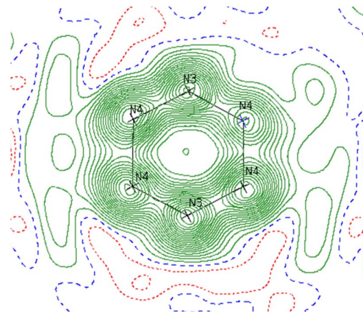
Fig. 6 Contour map of F obs for 5-Li showing the plane bisecting the Ti-Ti vector. Range: -0.60 to 3.80 e - Å -3 in steps of 0.20. Negative contours are shown in red and positive in green. Residual electron density outside of the N ring indicates likely partial occupancy of another atom at those positions.
