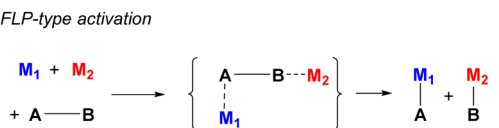
Scheme 3 Selected examples of various types of heterometallic cooperative bond activation.
