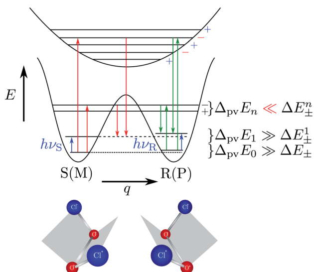
Fig. 23 Enantiomers of chiral molecules of the general type X-Y-Y-X and scheme for the experiment to measure \Delta_{pv}E (red arrows for time-dependent experiment) and \Delta_{pv}\nu = \nu_S - \nu_R (blue arrows). The combination of selected red and green arrows in the scheme leads to a measurement of \Delta_{pv}E in the frequency domain. The excited state of well defined parity (minus or plus signs) can be in an electronically excited state or in an excited vibrational-tunneling state as shown in ref. 231. The red arrow in absorption corresponds to a transition between an S and a negative parity level (energy h\nu_{S-} ). The green arrow in absorption corresponds to a transition between an R and a negative parity level (energy h\nu_{R-} ). The difference is h\nu_{S-} - h\nu_{R-} = \Delta_{pv}E_0 . The energy difference between the two blue absorption lines within R and S , h\nu_{S-} - h\nu_{R-} = \Delta_{pv}E_0 - \Delta_{pv}E_1 , is the difference of parity violating energy differences (modified after ref. 69 and 136).
