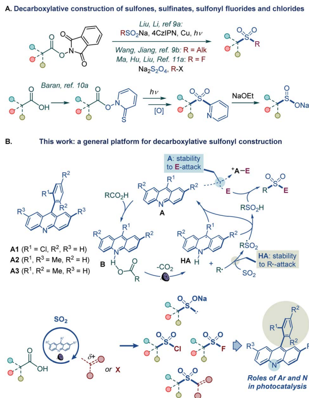
Fig. 2 (A) Decarboxylative construction of sulfones, sulfinates, sulfonyl fluorides and chlorides. (B) Functional group-divergent decarboxysulfonylation by acridine photocatalysis.
