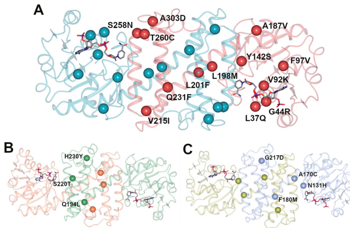
Fig. 5 (A) Model of structure of 'IR-46' derived using AoIRED (5FWN). 39 The model shows the location of amino acid residue sites that were mutated in variant 'M3,' applied in the kg-scale synthesis of 53n in Scheme 20; (B) structure of IRED88 (ref. 81) (PDB 7OG3) showing locations of residues mutated in variant Q194L/S220T/H230Y, used in the gram-scale synthesis of 54b in Scheme 21; (C) model of structure of SpRedAm 40 showing locations of residues mutated in variant 'R3-V6' used in the ton-scale synthesis of 58b (Scheme 22).
