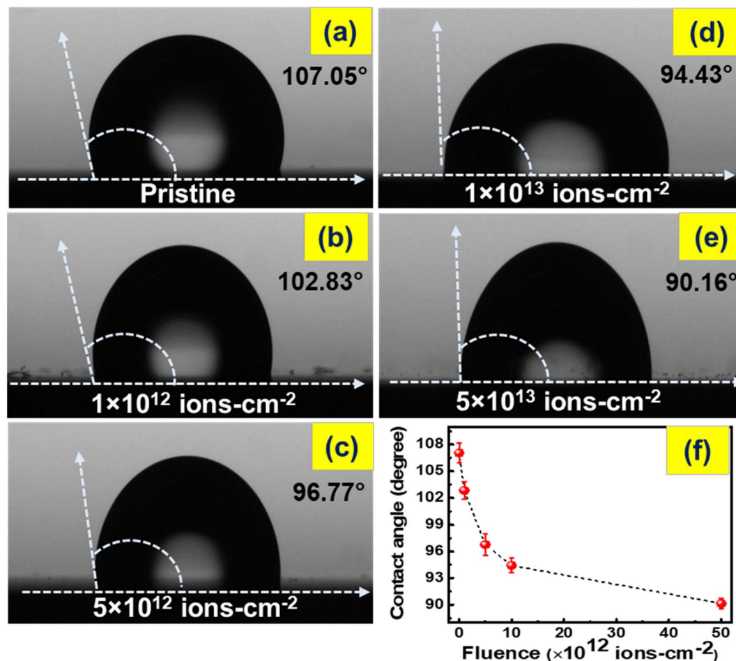
Fig. 14 Contact angles (CA) of (a) pristine film, and absorber films developed at different fluences of (b) 1 \times 10^{12} ions per cm 2 , (c) 5 \times 10^{12} ions per cm 2 , (d) 1 \times 10^{13} ions per cm 2 , and (e) 5 \times 10^{13} ions per cm 2 . (f) Variation of CA with ion fluence. [Reproduced/adapted from Maity et al. , 159 J. Appl. Phys. , 2021, 129, 045301, with the permission from AIP Publishing.]
