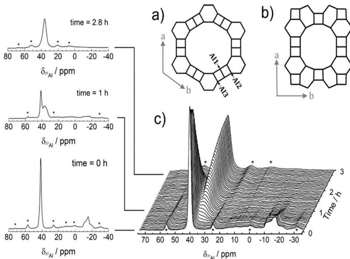
Fig. 22 (a) Structure of VPI-5 shown along c -direction, (b) structure of \text{AlPO}_4\text{-8} along c -direction. Alternating Al and P atoms are linked via oxygen atoms, the three crystallographically independent Al positions are marked in the figure. (c) In situ ^{27}\text{Al} MAS NMR spectra displaying the transformation of VPI-5 to \text{AlPO}_4\text{-8} (spinning with MAS rate of 2 kHz at 100 °C in a dry nitrogen flow). Asterisks denote spinning sidebands. (Reprinted with permission from ref. 119. Copyright © 2020, American Chemical Society.)
