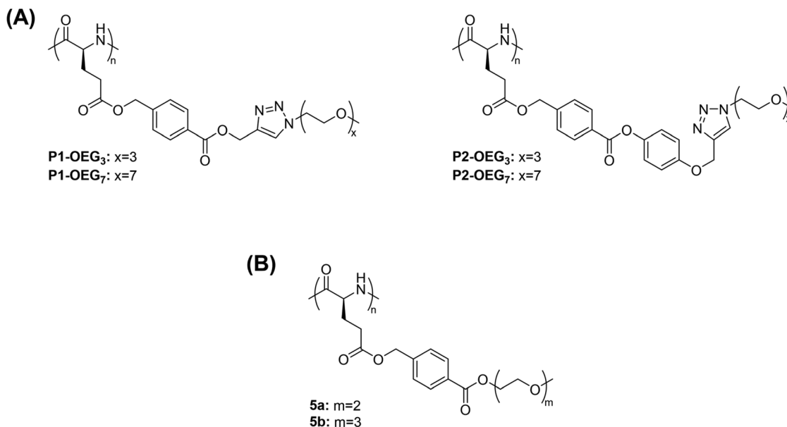
Fig. 3 Chemical structure of polypeptides with OEG pendants. (A) Polypeptides obtained by reacting poly( \gamma -4-(propargyloxybenzyl)-L-glutamate) ( P1 ) or poly( \gamma -4-(4-propargyloxyphenoxycarbonyl)benzyl-L-glutamate) ( P2 ) with azido functionalized OEG, 93 and (B) poly( \gamma -4-(2-(2-methoxyethoxy)ethoxycarbonyl)benzyl-L-glutamate) ( 5a ) and poly( \gamma -4-(2-(2-methoxyethoxy)ethoxy)ethoxycarbonyl) benzyl-L-glutamate). 98
