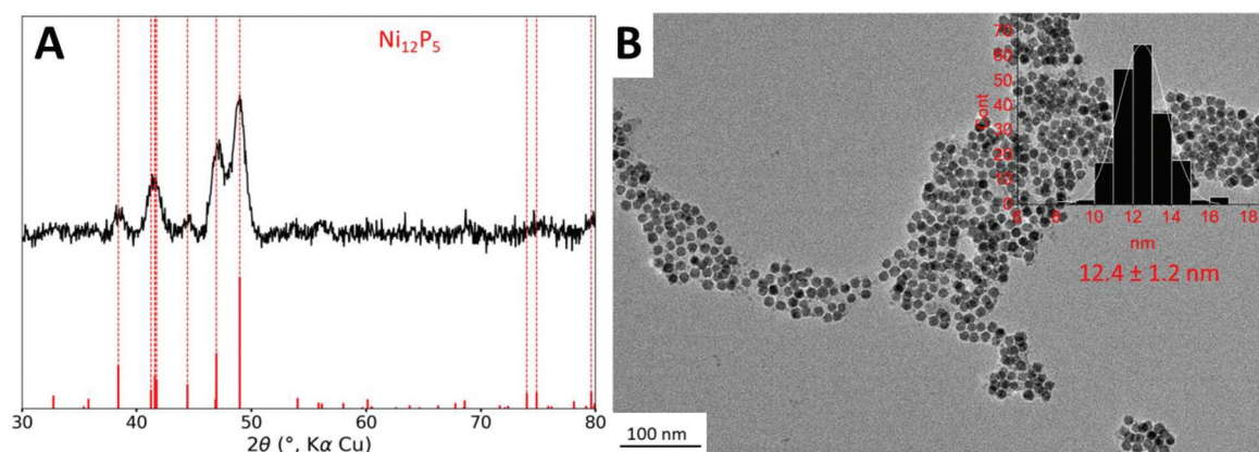
Fig. 1 (A) XRD pattern of the nanoparticles powder, the reference phase in red corresponds to \text{Ni}_{12}\text{P}_5 (PDF 03-065-4018, dotted lines are a guide to the eye). (B) TEM of the nanoparticles and size distribution in the inset.
