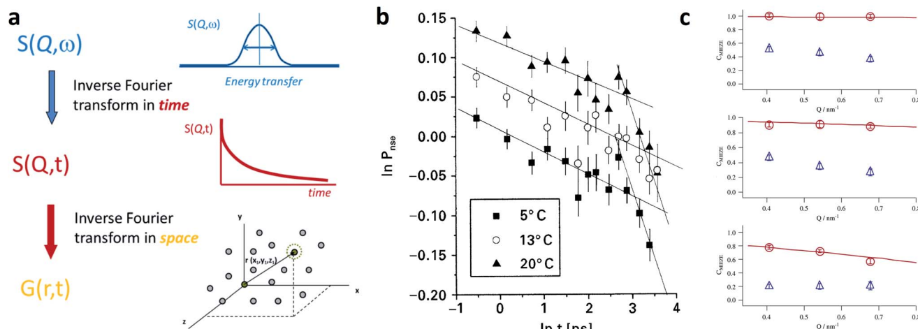
Fig. 13 (a) With time-of-flight and backscattering spectrometers the dynamic structure factor S(q, \omega) is detected, which can be converted by an energy Fourier transform into the intermediate scattering function S(q, t) , and which is directly measured by NSE. The time-dependent self-correlation function G(r, t) follows from a Fourier transform in space. With MIEZE the contrast C_{MIEZE} \propto \int S(q, \omega) \cos(\omega \tau_{MIEZE}) d\omega = S(q, \tau_{MIEZE}) is measured for a given MIEZE time \tau_{MIEZE} . Adapted from Arrighi and Higgins 365 under terms of the CC-BY license. (b) Lebedev et al. 357 determined the intermediate scattering function S(q, t) (here called P_{NSE} ) for a ferrofluid with 10 nm MnZn-ferrite MNPs at different temperatures. The NSE signal in double logarithmic scale clearly shows the existence of two distinct relaxation processes that scale with temperature. Copyright ©1999 Published by Elsevier B.V. (c) Hayashida et al. 364 investigated the relaxation dynamics of 10 nm magnetite MNPs in a ferrofluid by measuring the MIEZE contrast C_{MIEZE} of the nuclear (circles) and magnetic (triangles) scattering at three different q -values for three different MIEZE times (from top to bottom: 0.3 ns, 0.8 ns, 1.6 ns). The red line is the instrumental resolution function. The difference between nuclear and magnetic contrast can be attributed to the superparamagnetic relaxation of the MNPs. Copyright ©2008 Elsevier B.V. All rights reserved.
