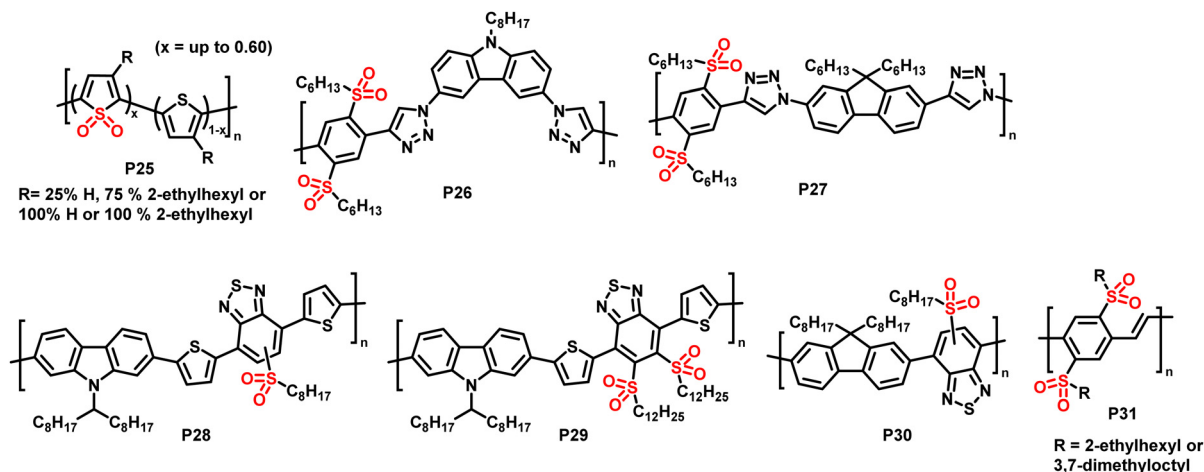
Fig. 12 Sulfone-substituted polymers P25–31 prepared via post-polymerisation oxidation of sulfur atoms in polythiophenes and alkythio-substituted polymers. 84–88
